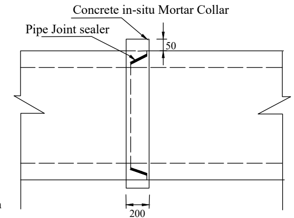
DETAIL OF PIPE JOINT
