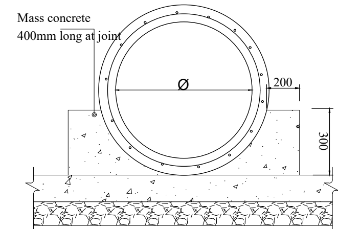
Detail concrete supporting pipe
