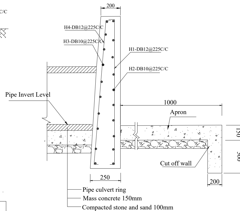
REINFORCEMENT DETAILS FOR HEAD WALLS
